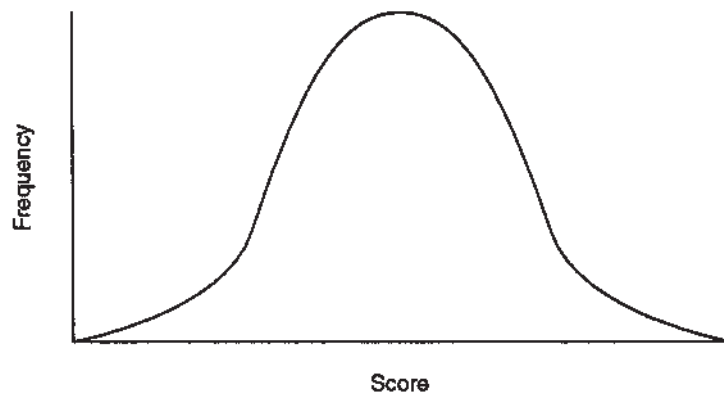
● Figure 1-6 The normal or Gaussian distribution.
