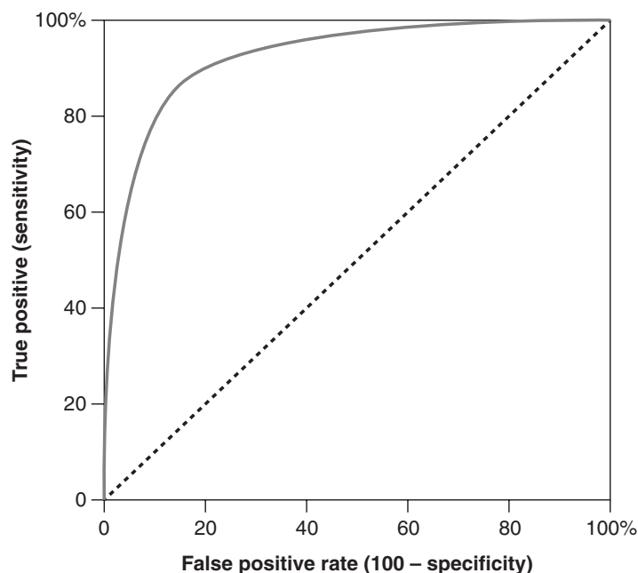
● Figure 7-4 Receiver Operating Characteristic (ROC) curve.
