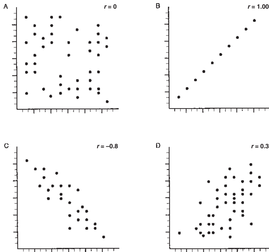
● Figure 4-1 Scattergrams.
