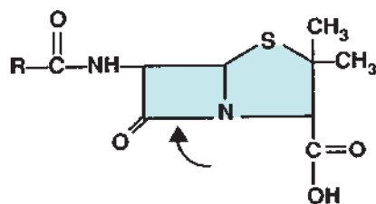
Penicillin nucleus
