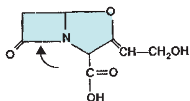
Clavulanic acid
