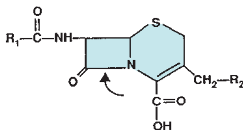
Cephalosporin nucleus
